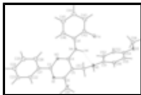
Fig. 1. Molecular structure of the title compound with displacement ellipsoids drawn at the 50% probability level and H atoms shown as small spheres of arbitrary radii. The dotted line indicates an intramolecular N—H···N hydrogen bond.
